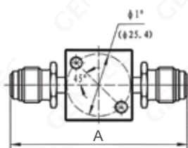
Face seal swivel male (FSR fittings)
